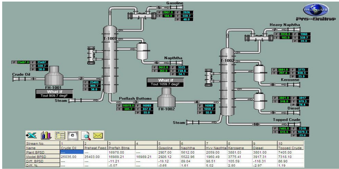
TYPICAL PRO-SCADA Graphic
